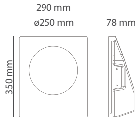
Dimensione foro 293x353 mm Cut hole sizes 293x353 mm
