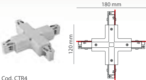
Cod. CTR4 Connettore a "X" "X" shape connector
