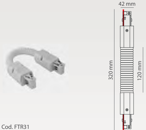
Cod. FTR31 Connettore flessibile Flexible connector
